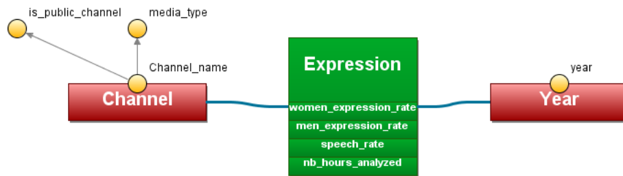
FIG. 9 – Final multidimensional schema
