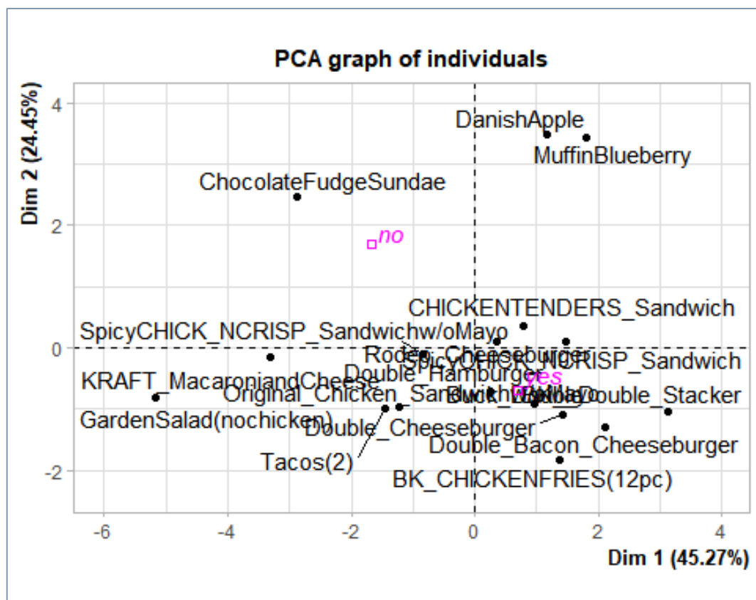
Figure 39 – Carte des individus – FactoMiner
