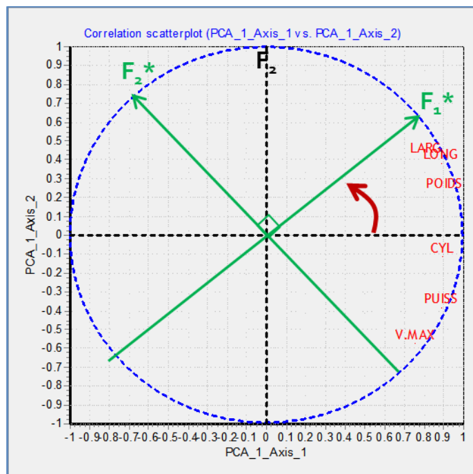
Figure 46 – ACP – Rotation VARIMAX – Cercle des corrélations
