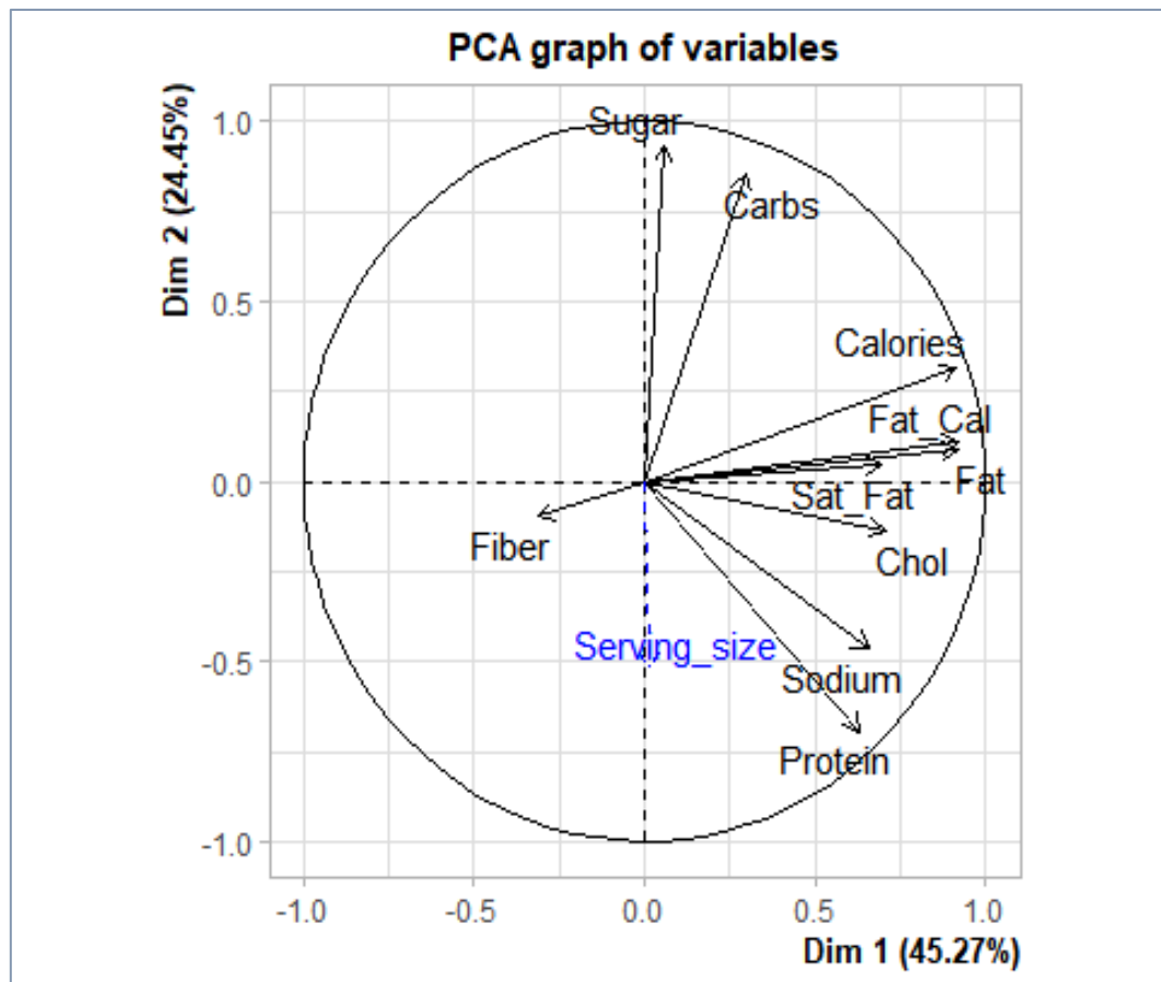
Figure 40 – Cercle des corrélations – FactoMineR
