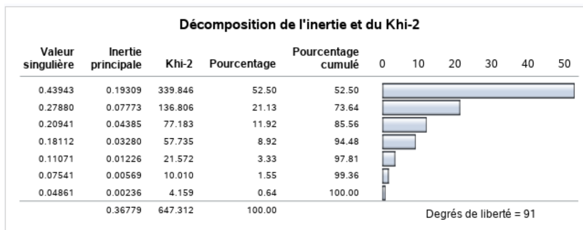
Figure 134 – Tableau des inerties – AFC – SAS PROC CORRESP
