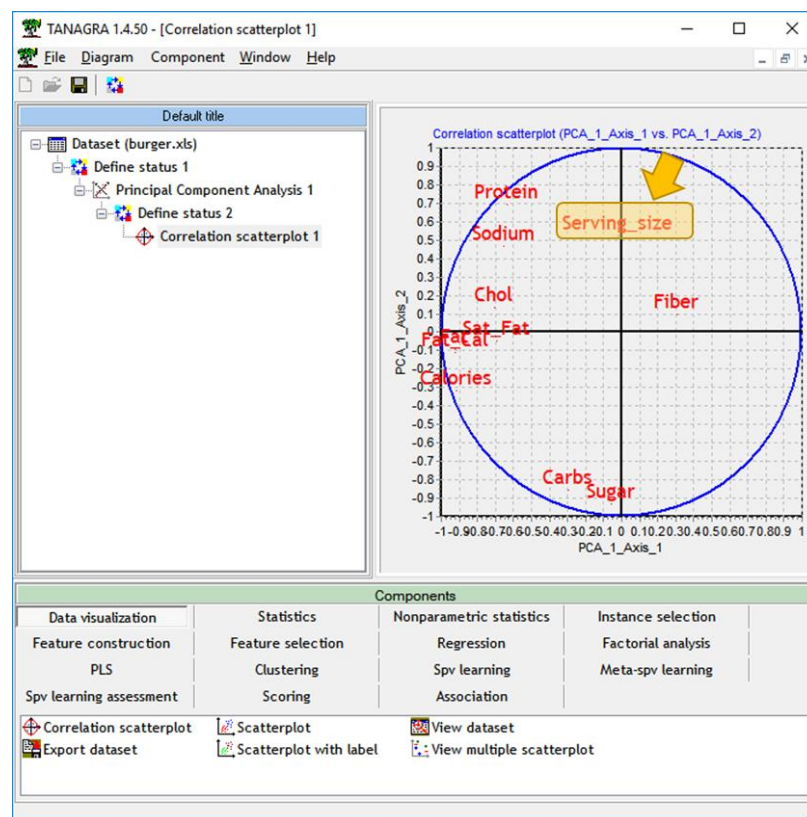
Figure 34 – Cercle des corrélations – Premier plan factoriel – TANAGRA
