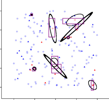
Fig. 2. Boundaries of the decision rules with ME^2 and a decision tree algorithm. The expressiveness of ME^2 is better to capture local specificities of the density function of the positives.
