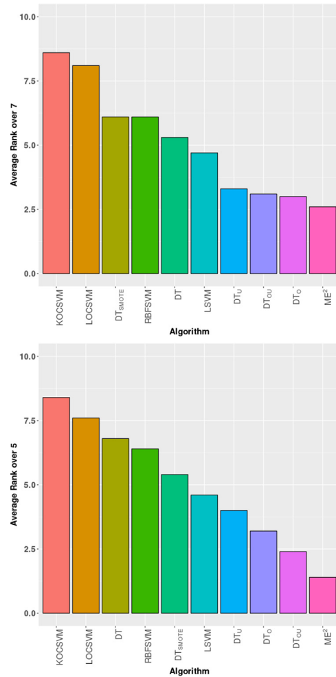
Fig. 3. Average ranks over all the datasets (top) and over the five most imbalanced datasets (bottom).
