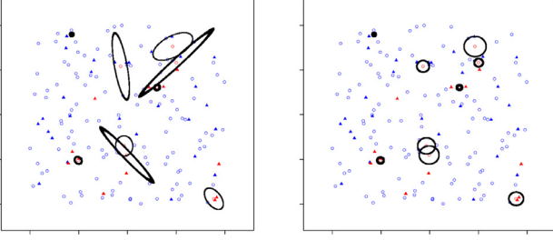
Fig. 1. Illustration of the interest of learning ellipsoids (on the left) rather than simple spheres (on the right). Optimizing the size and the orientation of the ellipsoids allows us to better capture local peculiarities.
