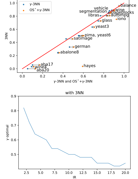
Fig. 6. (Top) Comparison of k -NN with (i) \gamma k -NN (points in blue) and (ii) \gamma k -NN coupled with the best sampling strategy ( OS^* ) (points in orange) for each dataset and for k = 3 . Points below the line y = x means that k -NN is outperformed. (Bottom) Evolution of the optimal \gamma value with respect to the IR for k = 3 .
