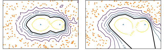
Fig. 3. Behavior of the decision boundary according to the \gamma value for the 1-NN classifier on two toy datasets. The positive points are represented by blue crosses and the negatives by orange points. The black line represents the standard decision boundary for the 1-NN classifier, i.e. when \gamma = 1 .
