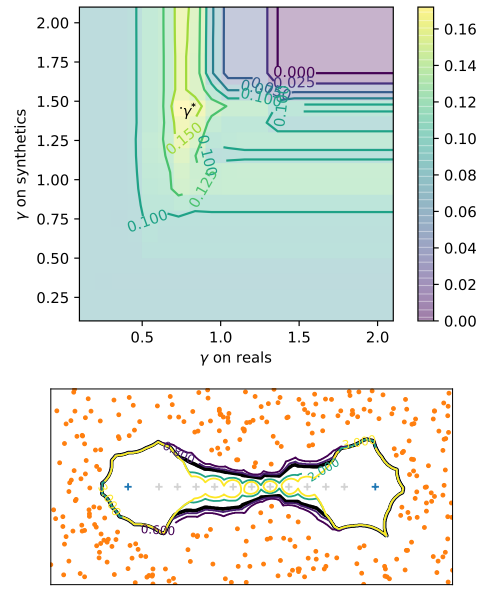
Fig. 5. (Top) An example of heatmap that shows the best couple of \gamma for the OS+\gamma k -NN strategy on the yeast6 dataset with SMOTE and Tomek's link. (Bottom) Illustration, on a toy dataset, of the effect of varying the \gamma for generated positive points (in grey) while keeping a fixed \gamma = 0.4 for real positive points.
