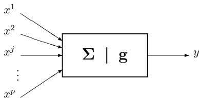
Figure 2: Neuron representation
