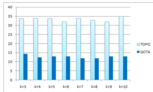
Figure 7: Comparison of the Runtime
