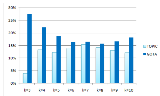
Figure 6: Comparison of the F-measure
