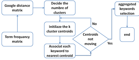
Figure 3: Steps of GOTA run.
