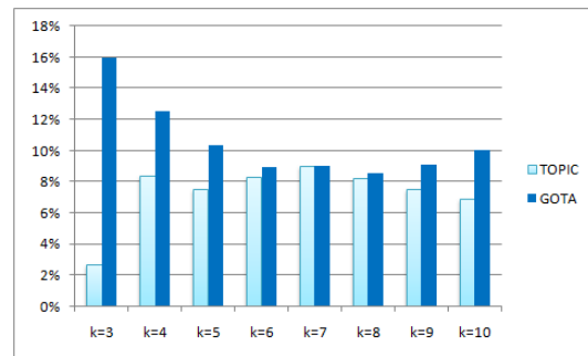
Figure 5: Comparison of the Precision
