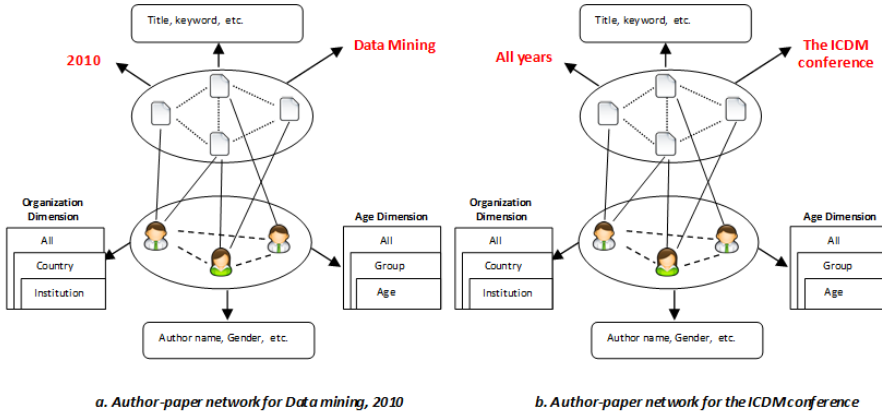
Fig. 4 Example of networks
