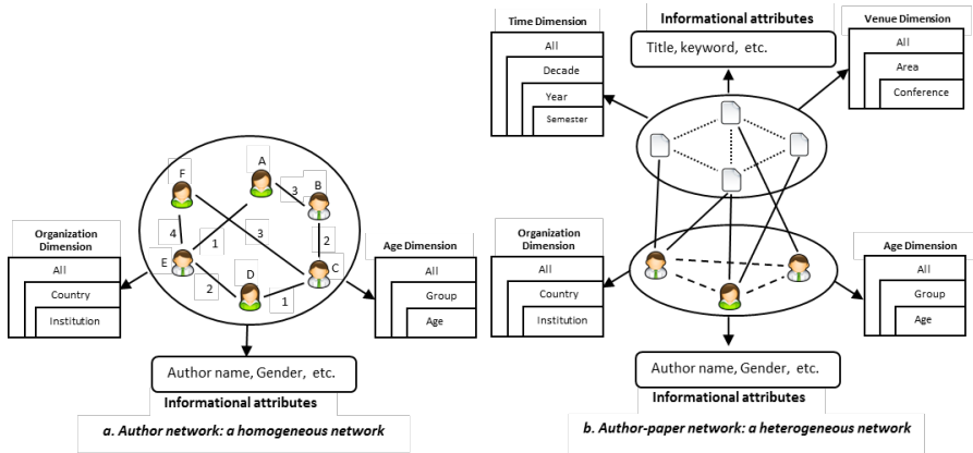
Fig. 1 Examples of bibliographic networks
