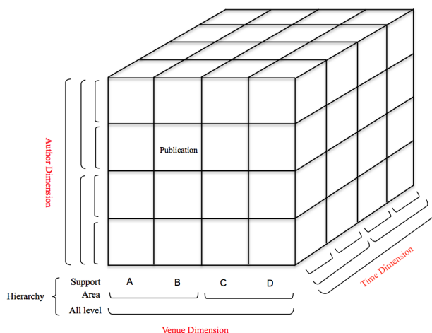
Fig. 2 Example of an OLAP cube
